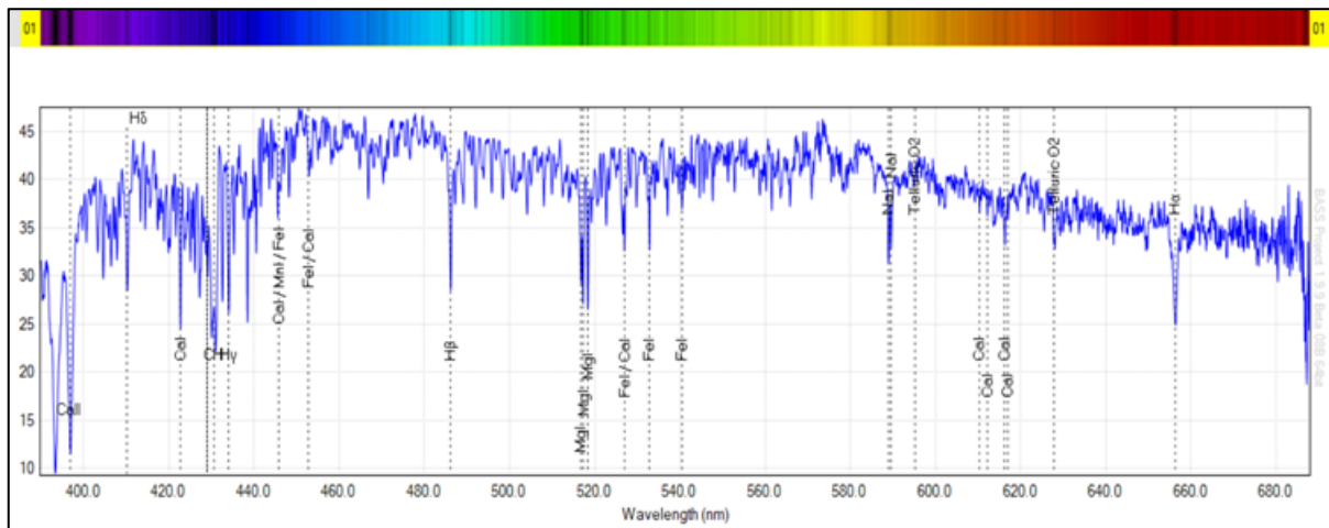
Fig 3. Solar spectrum for comparison.
