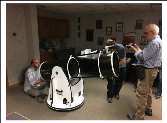
Fig 1. Preparing a 16-inch telescope for the 3 June occultation.
