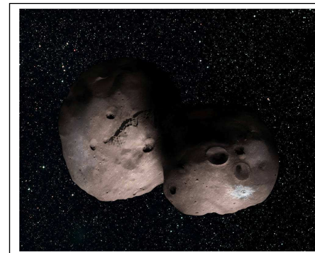
Fig 2. One artist's concept of 2014MU69. Credits NASA JHU APL SWRI Alex Parker.
