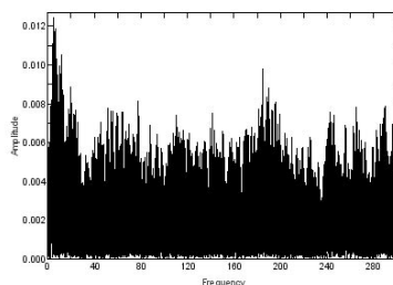
Figure 6: BS Tel after prewhitening of 3 frequencies.
