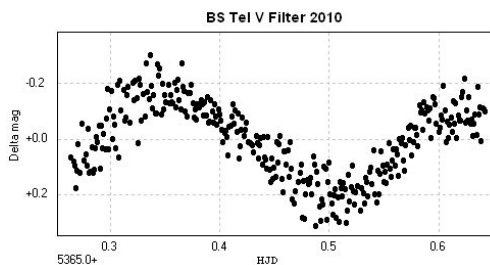
Figure 3: A typical night's observation.
