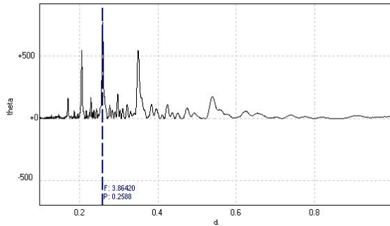
Figure 4: BS Tel V Filter Peranso primary period of P = 0.2588d
