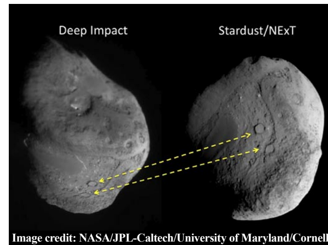
These two images show the different views of comet Tempel 1 seen by NASA’s Deep Impact spacecraft (left) and NASA’s Stardust spacecraft (right). Two craters, about 300 meters in diameter, help scientists locate the area hit by the impactor released by Deep Impact in July 2005. The dashed lines correlate the features.
