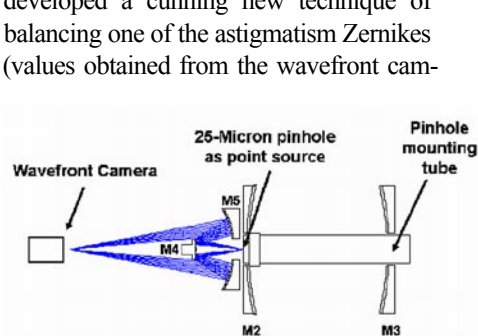
Fig. 3: The optical layout of the M4/M5 wavefront test. A pinhole positioned below the hole in M5 illuminates M4 and then M5 before forming an image on the wavefront camera.
