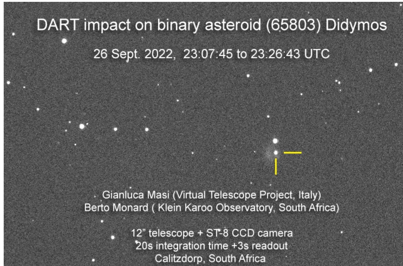
Fig 3. Dimorphos after impact showing the beginnings of a dust cloud around it.
