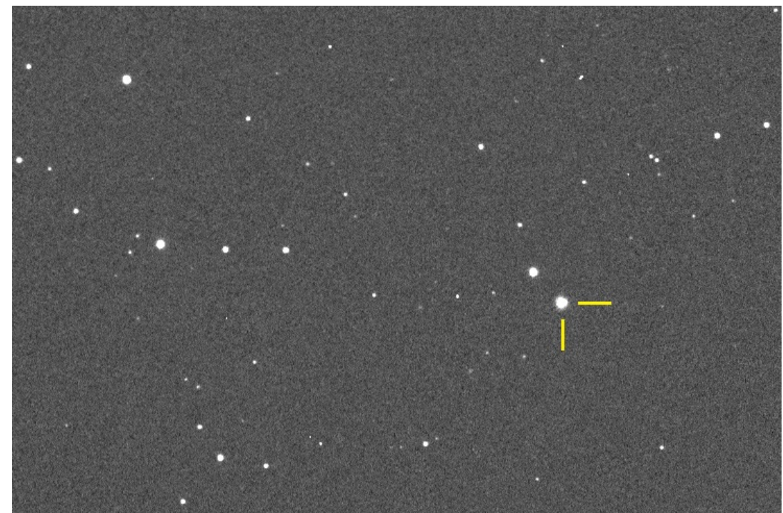
Fig 2. Marked brightening of Dimorphos during impact
