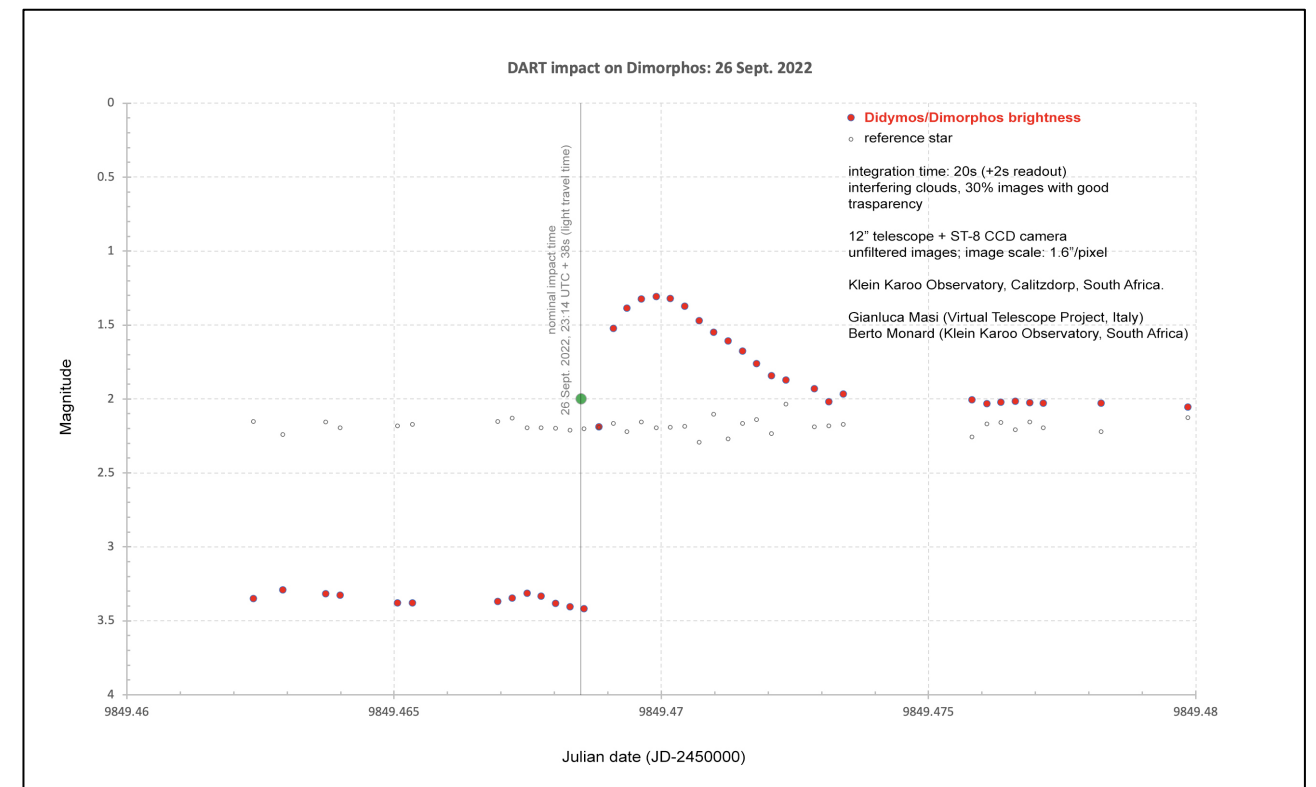
Fig 4. Photometry of the event.
