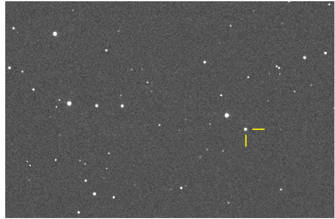
Fig 1. Dimorphos approaching Didymos; about 5 minutes before impact
