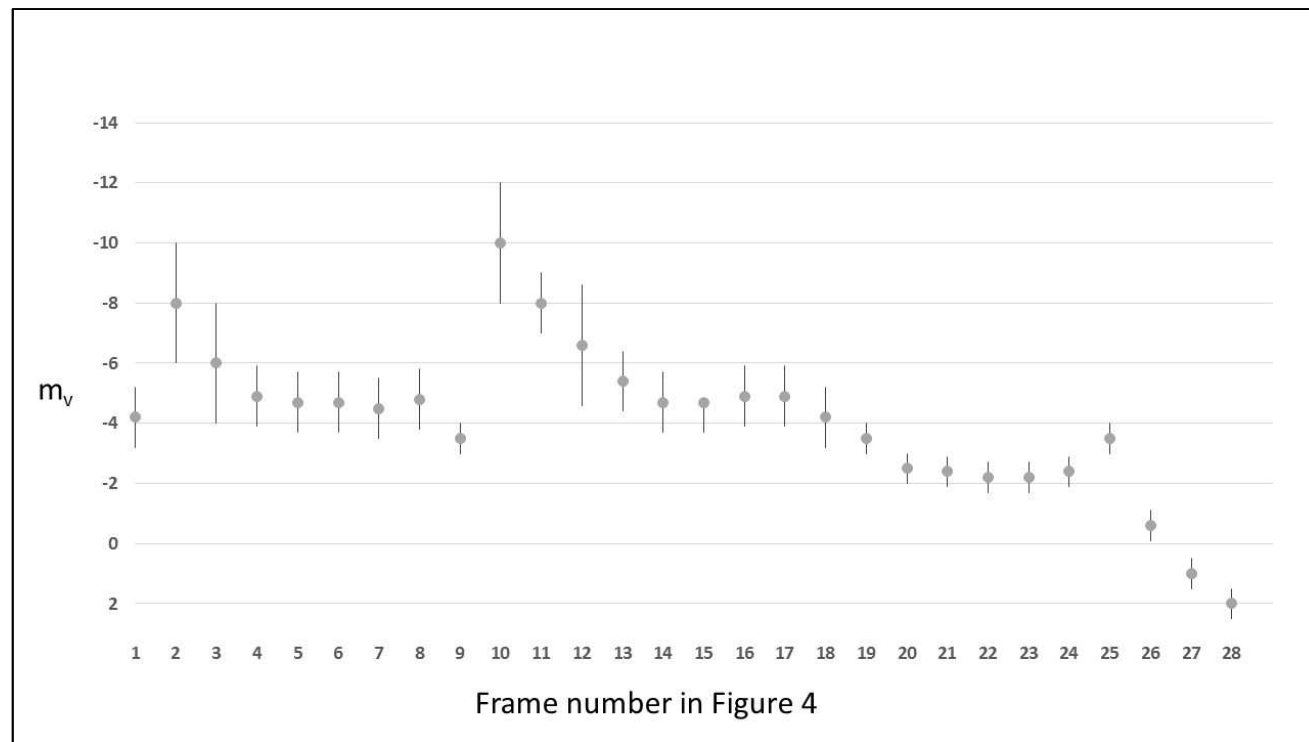
Fig 6. Light curve for Event 367. The fireball enters the field of view already bright, followed by flares in frame 2 to m_v = -8 and frame 10 when the brightness peaked at about m_v = -10 \pm 2 . Following fragmentation and another brief flare, the remaining fragments faded quickly from view. Error bars are larger and the brightness uncertain during peak brightness due to the lack of suitable comparison objects captured under the same exposure conditions. Error bars are smaller when the fireball was fainter due to comparison with Mars at similar brightness.
