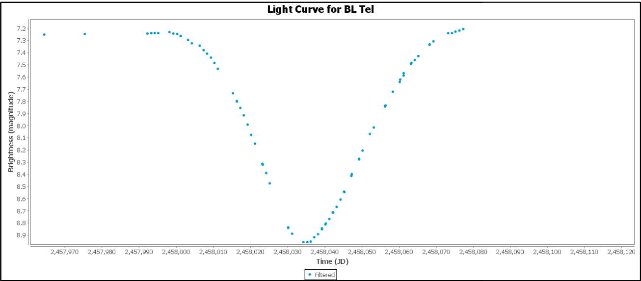
Fig 1. Light curve for BL Telescopii showing the 2017 eclipse.
