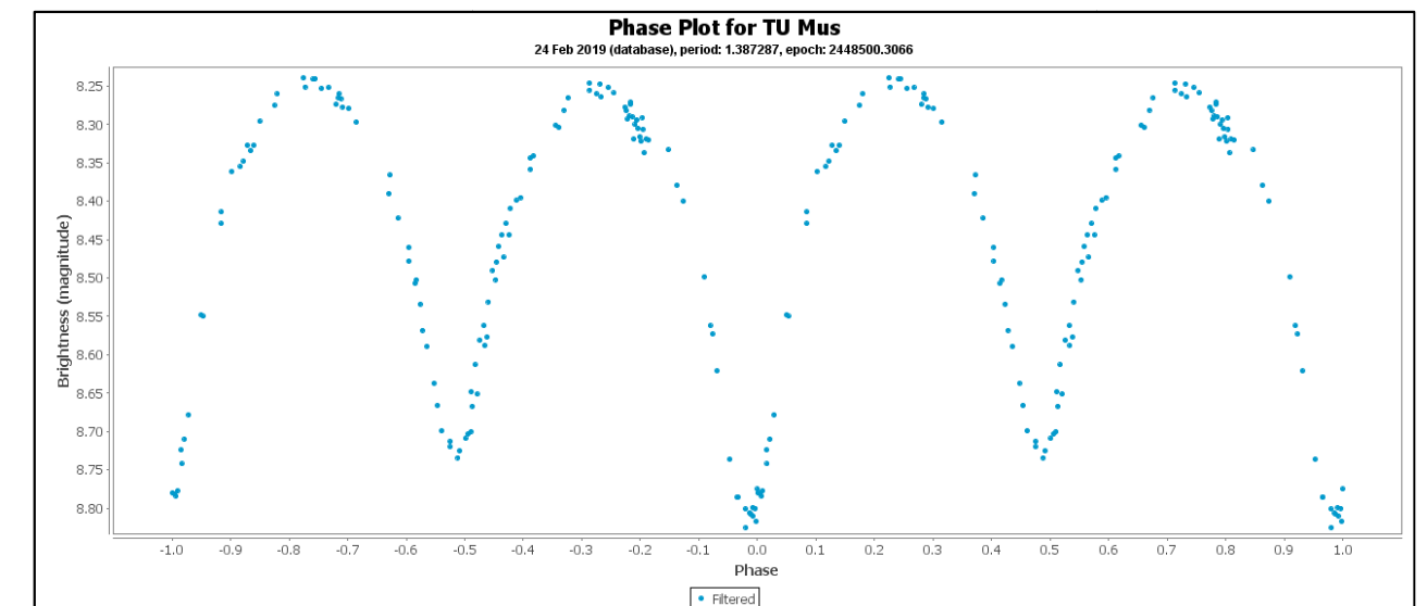
Fig 2. Phase plot of TU Muscae
