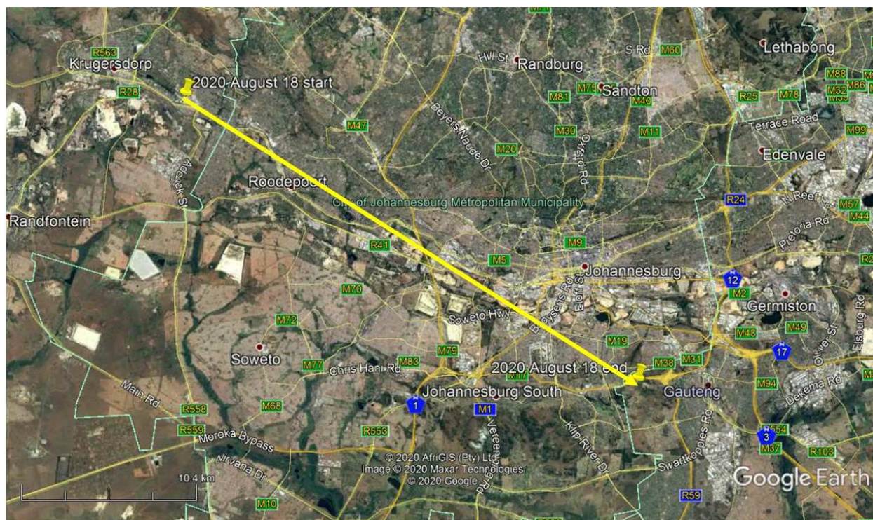
Fig 2. Ground path of Event 364, ablation started 88 km above a point just east of Krugersdorp and ended at 58 km above Alberton, about the location of the N12/R59 Reading Interchange.
