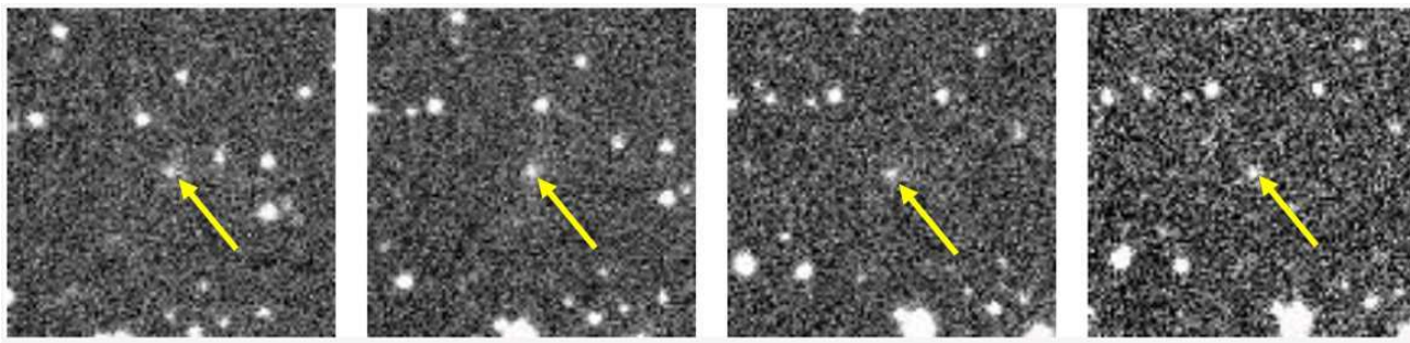
Fig1. The four 30 second exposures taken on Sep 17 UT by ATLAS-MLO at Mauna Loa, Hawaii.
