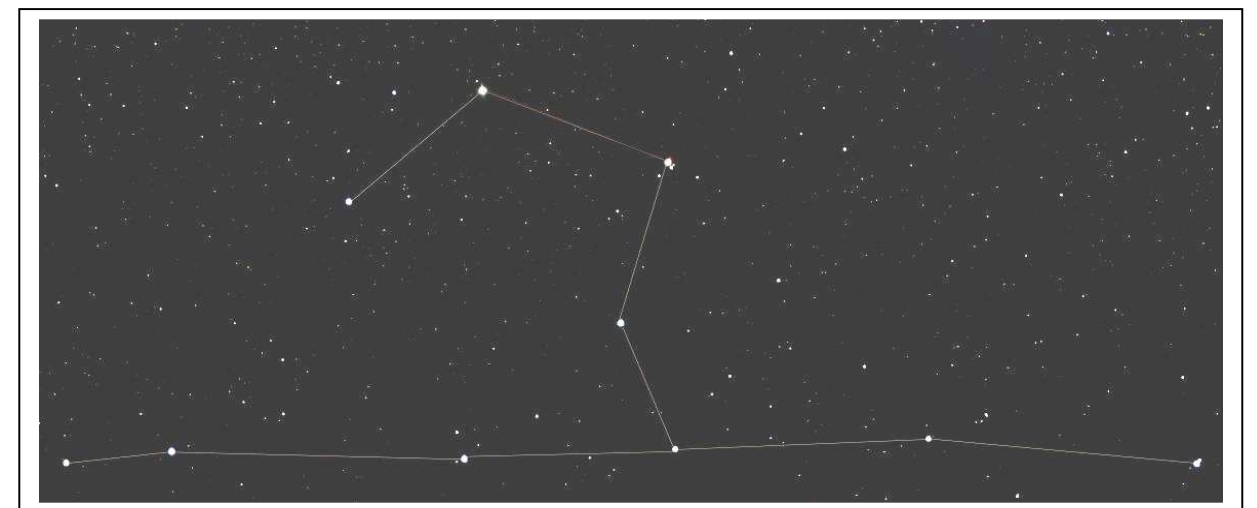
Fig 3. The Coathanger asterism (courtesy Dale Liebenberg)
