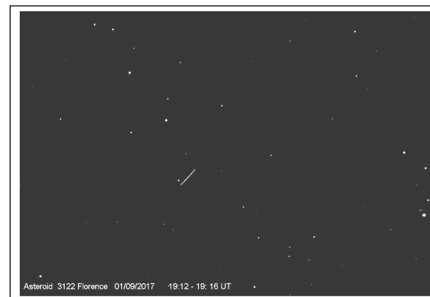
Fig 11. Asteroid 3122 Florence, Image by Oleg Toumilovich, 1 September, 2017, stack of 30 images showing motion from 19h12-19h16 UT, Canon EOS-550D camera set at ISO800, 20cm Celestron f/10 telescope. South is towards the top and
