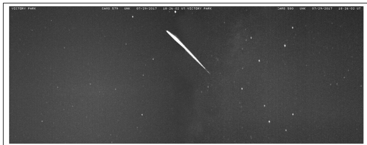
Fig 7. Possible fireball captured by two cameras at Victory Park. The two images have been aligned and joined to show the full path of the meteor. The constellation of Sagittarius is clearly visible to the right of the meteor.
