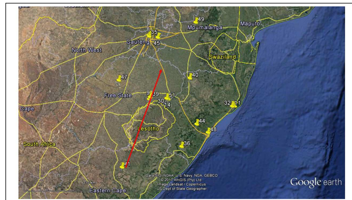
Fig 2. Locations of important reports, from which conclusions were arrived at to determine probable path (red arrow).
