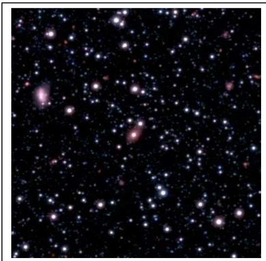
Fig. 2 An image of the galaxy SAGE0536AGN, from the Vista Magellanic Clouds survey. The galaxy is the elliptical object in the centre of the image. (Credit: Vista Magellanic Clouds survey)
