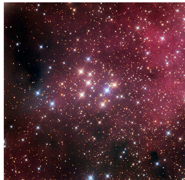
Fig 3. The open cluster M29.
