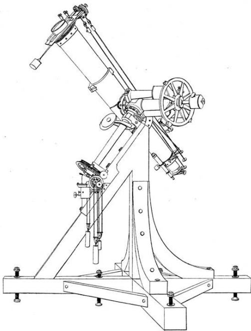
Fig. 3 The heliometer used by Bessel. The objective consisted of two semicircular lenses that could be moved very precisely relative to each other and also rotated. This enabled the angle between two stars to be measured very precisely.
