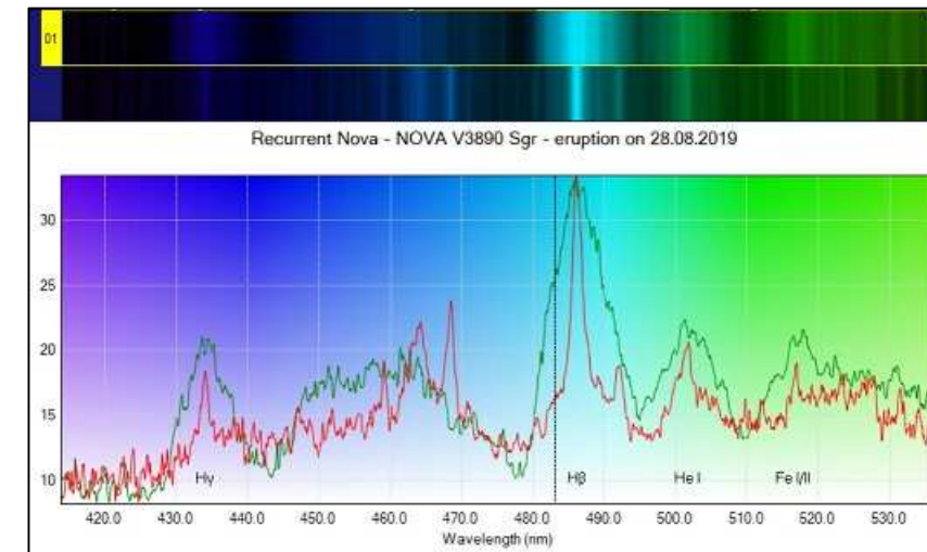
Fig 13: 2nd-time mag.~>8.5 – 03.09.2019
