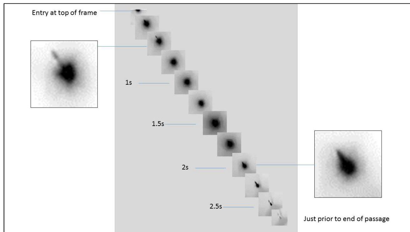
Fig 3. Event 349 – 2020 May 31 at 18h26, appearance of fireball in intervals of 0.25 seconds in CCTV footage. Fireball is already bright as it enters the frame at top left. Peak brightness occurs at 1.5 seconds into the clip. Enlargements show differences in appearance before and after peak brightness.
