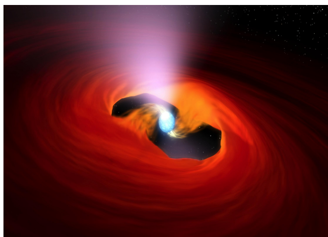
Fig 1. An artist's depiction of an accreting pulsar. Image: NASA
