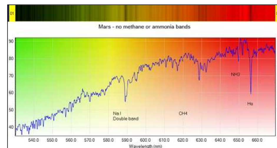
Figs 6 – 8: (top to bottom) Jupiter & Saturn show a strong band of Methane and a weak band of ammonia. Mars shows no methane or ammonia
