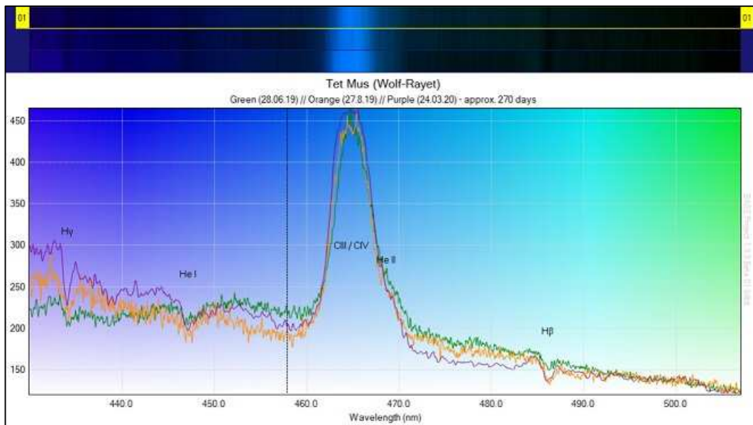
Fig 19: Blue spectra of θ Mus at three epochs.
