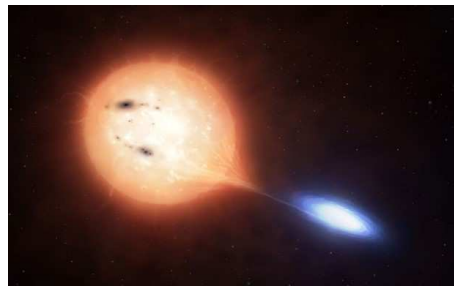
Fig 9. Artist's impression of SS Lep
