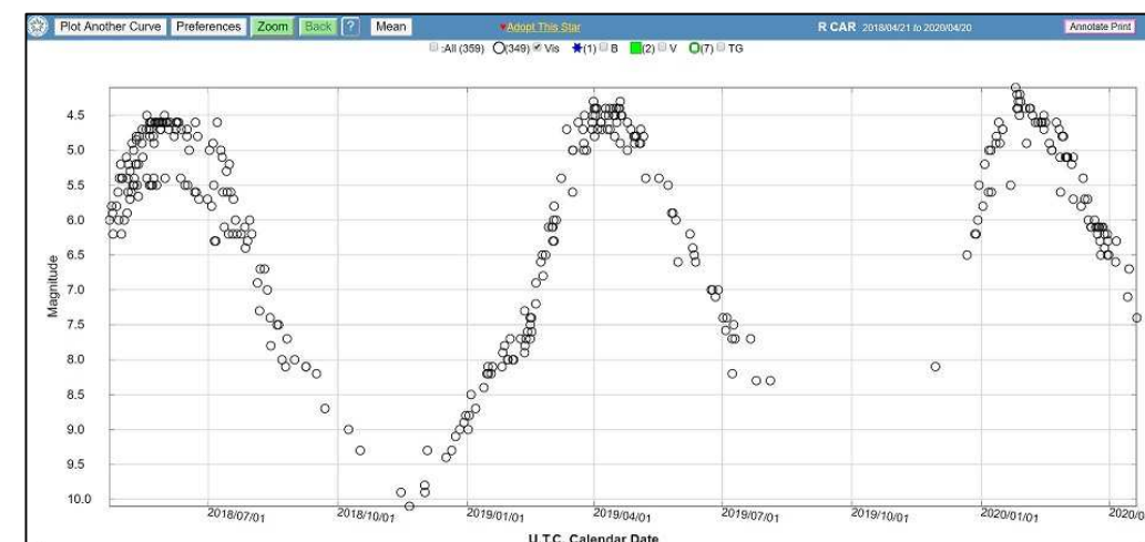
Fig 16: Light curve of R Car (AAVSO)
