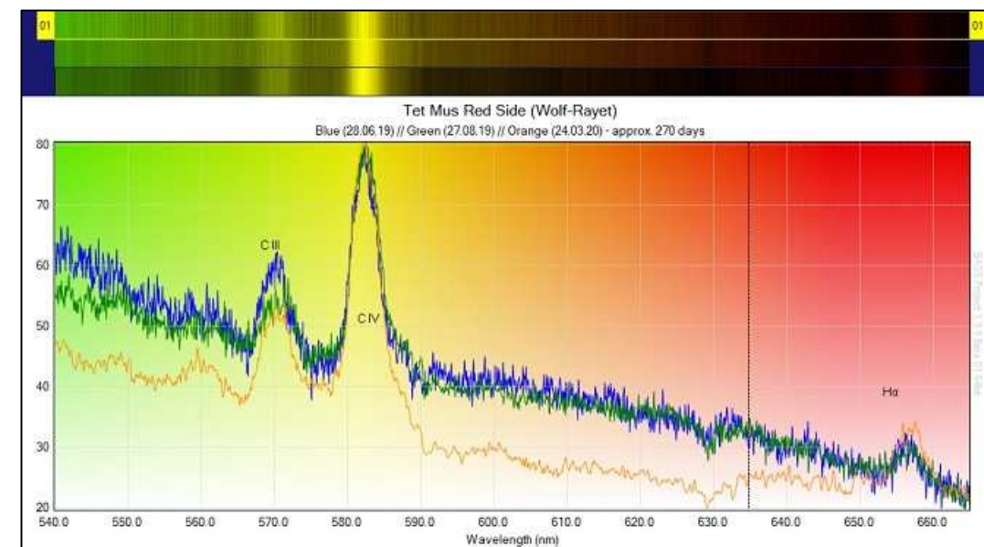
Figs 19 & 20 ∅ Mus on three dates in two spectral regions.
