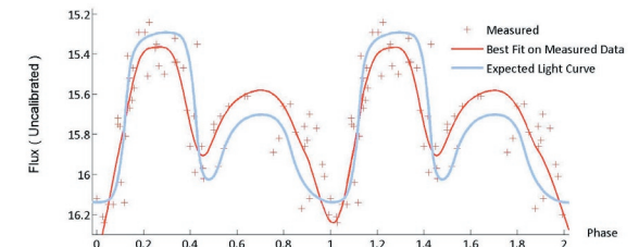
Fig.10 The Crab Pulsar light curve compiled from 12 hours of photometric measurements during Jan/Feb 2013. The Cycle was repeated for illustration.
