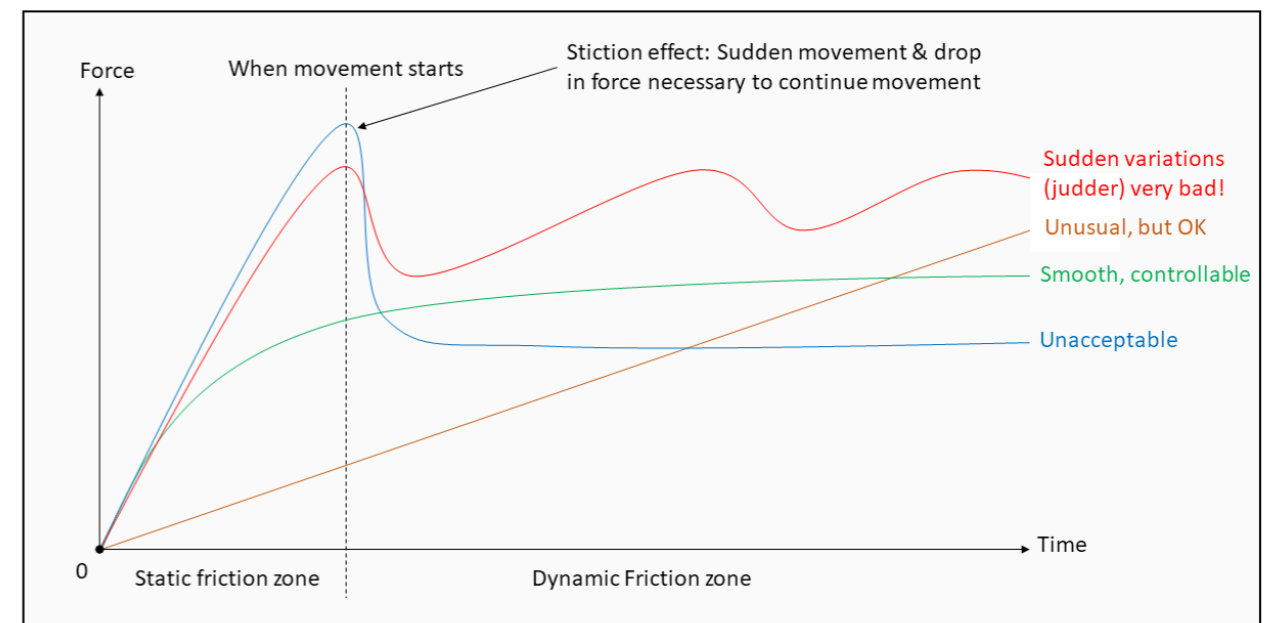
Fig 1. Friction effects on smoothness of movement.
