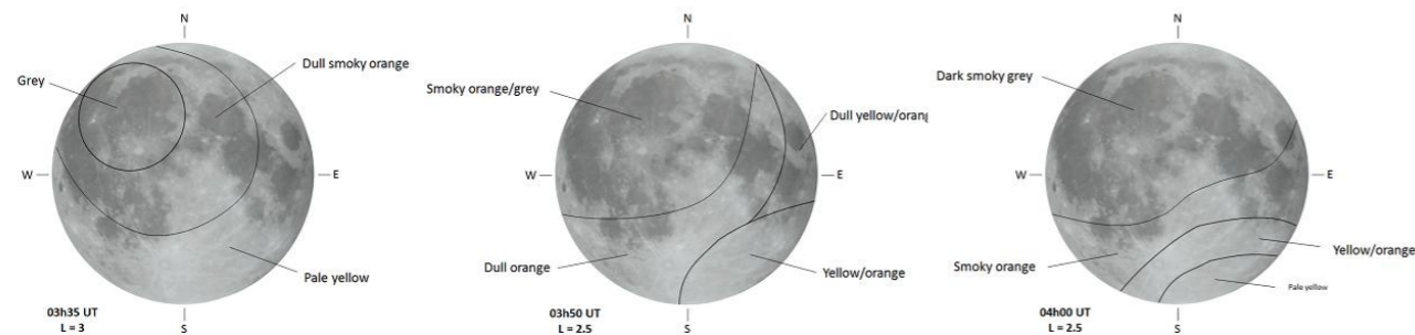
Fig 6. Visual observations of colour by the author. Note directions are in selenographic coordinates. Observations made using 16x50 binoculars.
