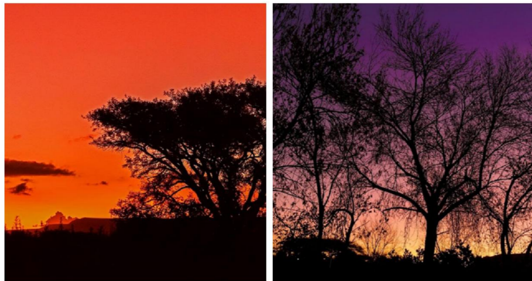
Fig 5. Images of brightly coloured sunsets by Angus Burns, Newcastle, KZN, following the eruption of HTHH on 15 January 2022. Left image taken on 22 February 2022, Canon 5D Mark IV, 24-70mm F4L IS USM lens, ISO800, f/4.5, 1/15 second exposure. Right image taken on 16 June 2022, Canon 5D Mark IV, 24-70mm F4L IS USM lens, ISO400, f/4, 1/30 second exposure. Both images unprocessed.
