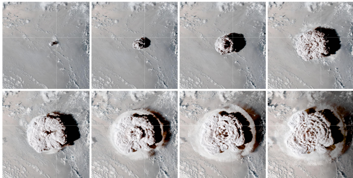
Fig 4. Sequence of images of eruption of HTHH on 15 January 2022, starting upper left at 04h10 UTC, to lower right at 05h20 UTC. From measurement of shadow lengths the plume was ascertained to reach an altitude of 58 km, extending into Earth's mesosphere. NASA Earth Observatory images and by Joshua Stevens, using data courtesy of Kristopher Bedka and Konstantin Khlopenkov/NASA Langley Research Center, and GOES-17 imagery courtesy of NOAA and the National Environmental Satellite, Data, and Information Service (NESDIS).
