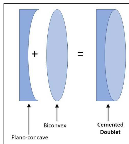
Fig 4. Cemented Doublet
