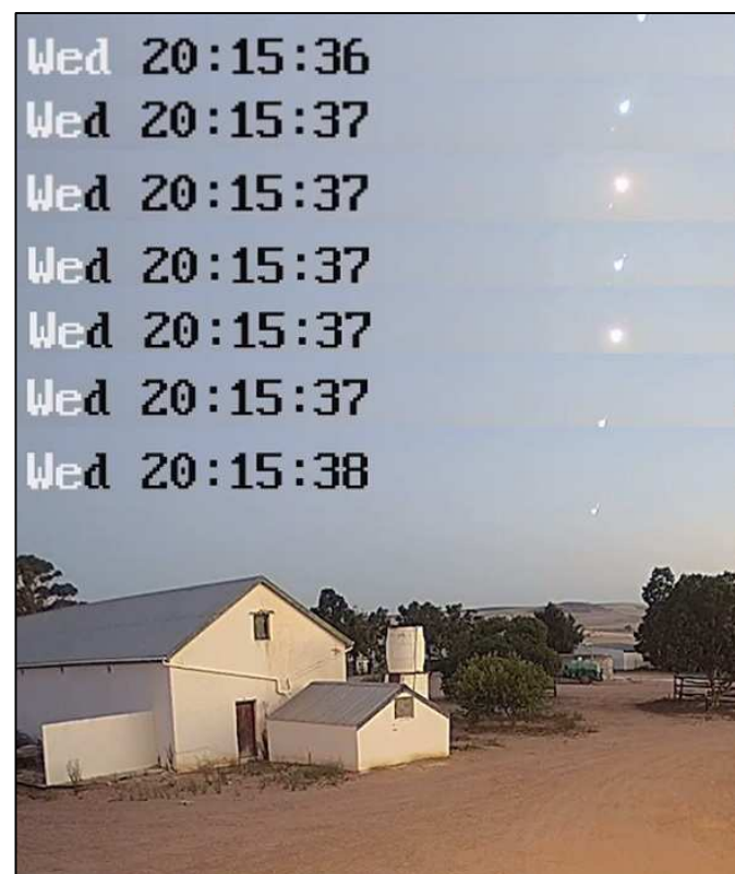
Fig 4. Sequence of frame grabs from Malmesbury video footage. Top frame is the first appearance of the bolide at upper right. The third and fifth frames show the two explosions. Last frame is immediately before the bolide ceases to be visible. In some frames at least three fragments are visible. Note total flight time in the Malmesbury video is just under 2 seconds, and the two explosions are separated by less than 1 second.
