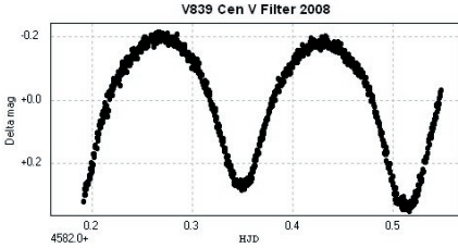
Figure 4: V 839 Cen V Filter 2008
