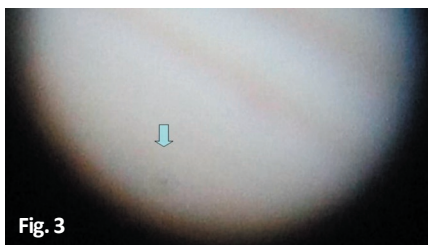
Fig. 1-3: Enlarged images, taken between 20:48 and 20:49, showing the shadow appearing as a faint dot (arrowed) with a faint circle (the penumbra) around it, moving along the edge of the Jovian disk.
