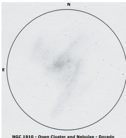
NGC 1910 - Open Cluster and Nebulae - Dorado
