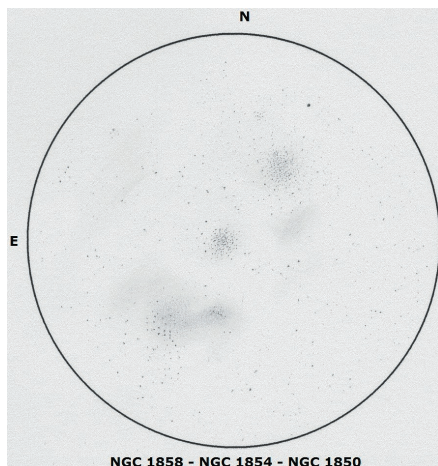
NGC 1858 - NGC 1854 - NGC 1850
