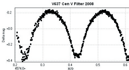
Figure 6: V637 Cen V Filter 2008
