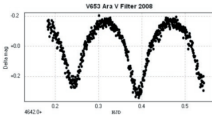
Figure 8: V653 Ara V Filter 2008.
