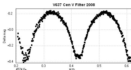
Figure 6: V637 Cen V Filter 2008
