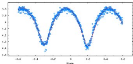
Figure 7: V637 Cen V Filter 2008. Fitted synthetic light curve (solid line) on phase binned light curve.
