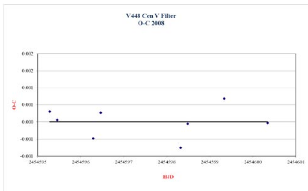
Figure 2: O-C graph of V448 Cen V Filter 2008 season. Points 1, 3, 5, 7 and 8 are secondary minima.
