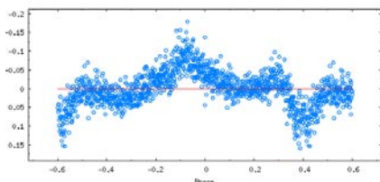
Figure 3: V448 Cen V Filter 2008. Fitted synthetic light curve (red) on binned light curve.
