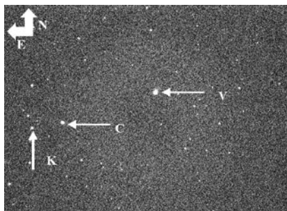
Figure 1: V839 Cen (V) and Check (K) and Comparison (C) star
