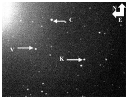
Figure 2: V637 Cen (V) and Check (K) and Comparison (C) star
