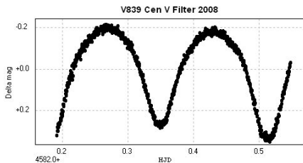
Figure 4: V 839 Cen V Filter 2008
