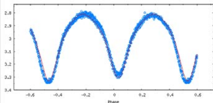
Figure 5: V 839 Cen V Filter 2008. Fitted synthetic light curve (solid line) on phase binned light curve.
