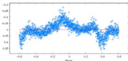
Figure 4: V448 Cen residuals of the PHOEBE model.
