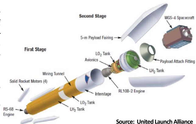
Fig. 1: Details of the rocket stages and payload are shown here. The fuel dump originated from the 2 nd stage after payload separation.
