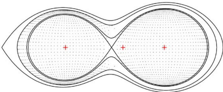
Figure 5: Roche lobe fillout of V448 Cen at 0.15 of phase.
