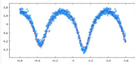
Figure 9: V653 Ara V Filter 2008. Fitted synthetic light curve (solid line) on phase binned light curve.
