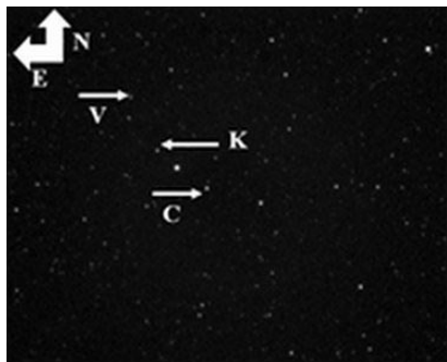
Figure 3: V653 Ara (V) and Check (K) and Comparison (C) star
