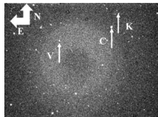
Figure 1: V448 Cen (V) and Check (K) and Comparison (C) star.
