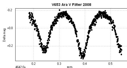
Figure 8: V653 Ara V Filter 2008.
