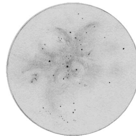
NGC 2070, the Tarantula Nebula
