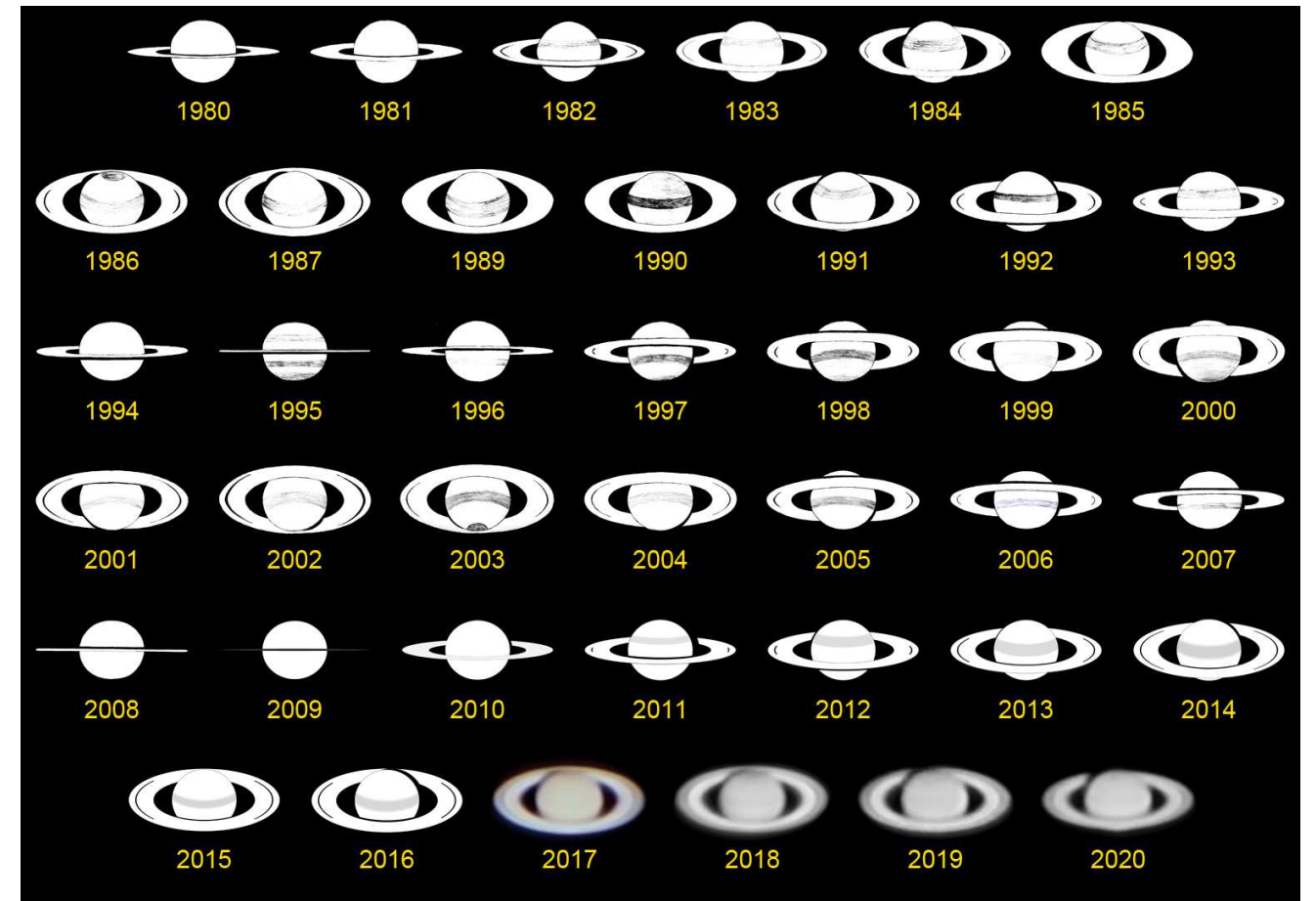
Fig.1. Saturn between 1 November 1980 and 2 November 2020. North is up and east to the left.
