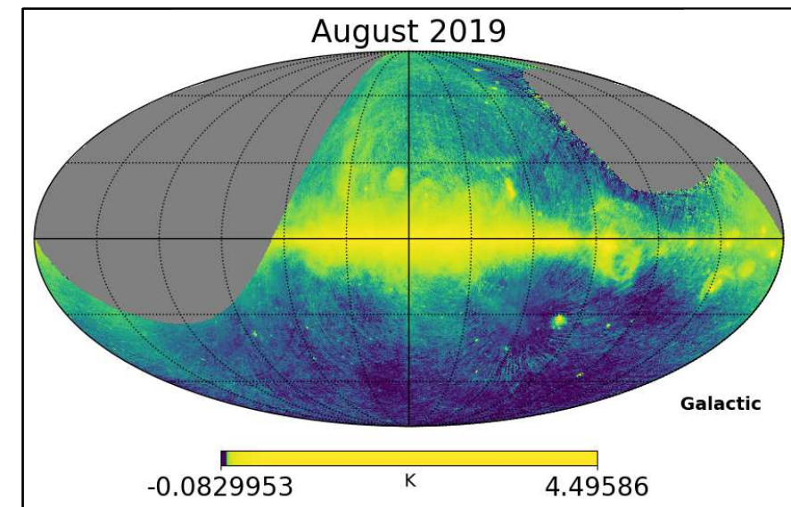
Fig 10. The Southern hemisphere data from C-BASS at 6cm to date. Most of this is “Synchrotron Radiation” whose effects extend to the mm-region wavelengths observed by the Planck satellite). The bar at the bottom is “antenna temperature”, a measure of brightness used by radio astronomers (courtesy Prof J Jonas, Rhodes University).
