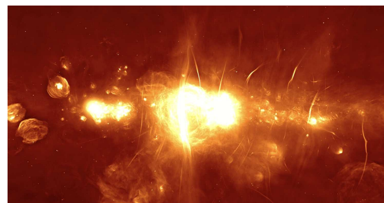
Fig 6. MeerKAT radio image of a 2° x 1° region around the Galactic Centre. Especially notable are the many filaments, a manifestation of synchrotron radiation from high-energy electrons spiraling along magnetic field lines (Photo: MeerKAT, SARA0).
