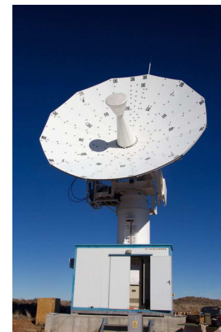
Fig 11. The C-bass antenna at Klerefontein near Carnarvon. It has a diameter of 7.6m and was donated by Telkom.
