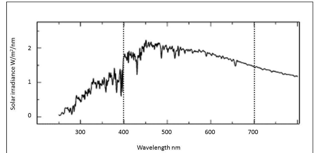
Fig. 1 Low resolution extra-terrestrial solar spectrum (Chance 2005).
