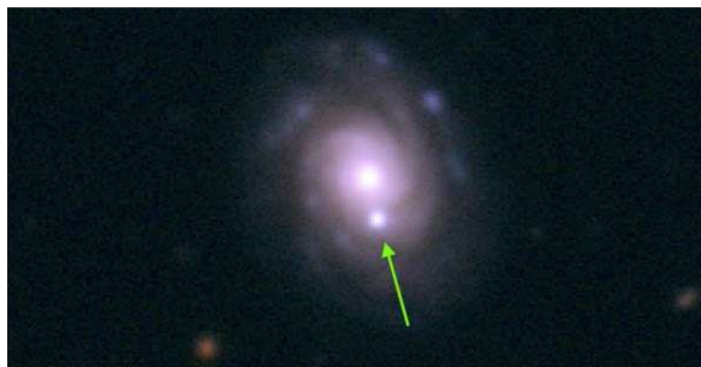
Fig. 2 Zoomed in and rotated image of the supernova in Figure 1, highlighting it in one of the host galaxy’s spiral arms. For a brief time the supernova can be as bright as the 100 billion stars of the host galaxy. Image Credit: SALT/SAAO
