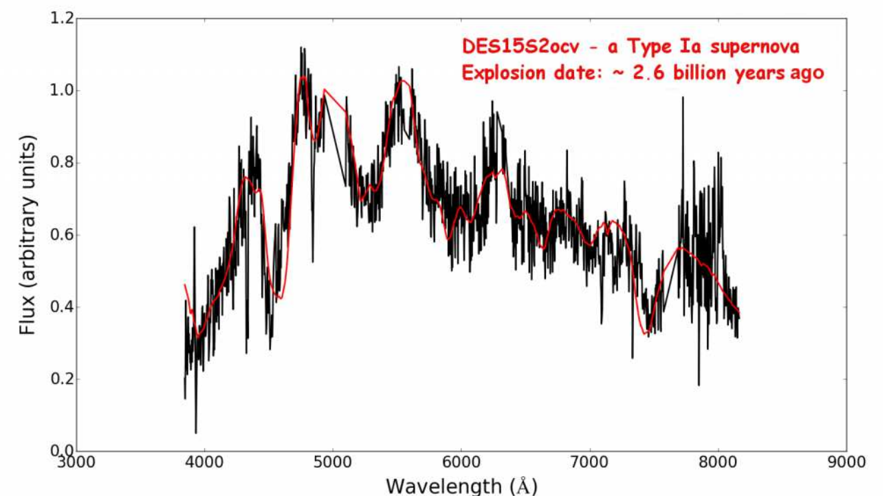
Fig. 3 A spectrum of the Type Ia supernova “DES15S2ocv” taken by SALT on the 9th of January 2016. Over-plotted in red is a template spectrum used to classify the supernova. Image Credit: SALT/SAAO
