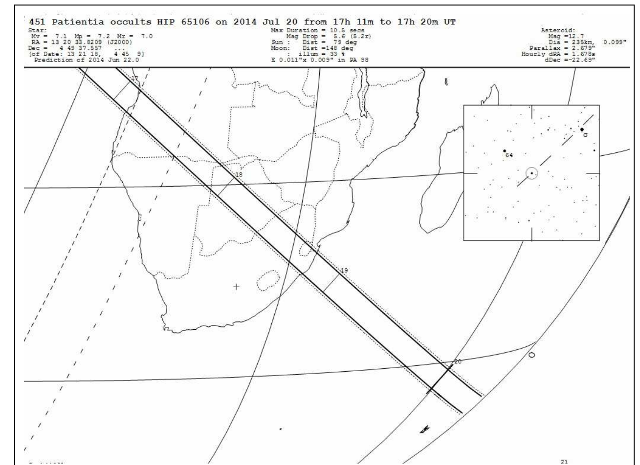
Fig 2. Asteroid Patientia's track across southern Africa.
