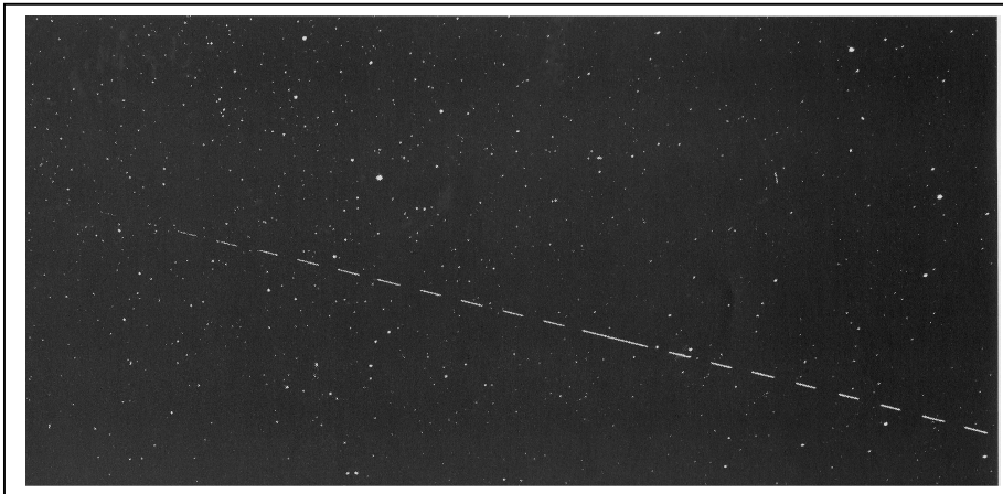
Fig 1. Image of Sputnik 1 casing.
