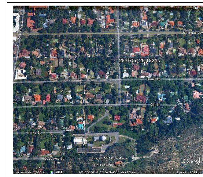
Fig 4. Google earth location of Johannesburg MOONWATCH which should be at bottom edge of the image.
