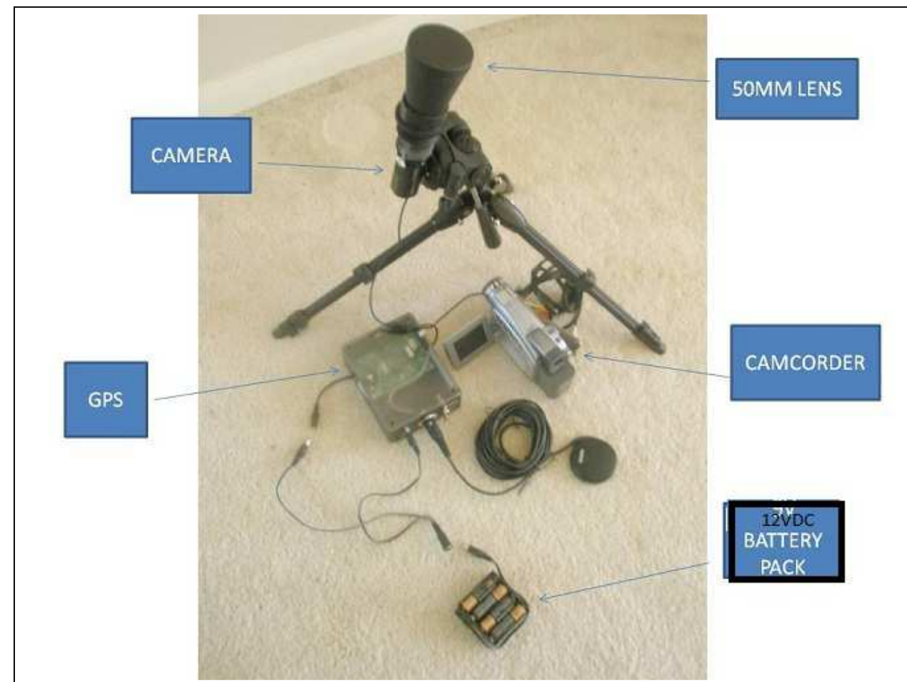
Fig.1. Typical equipment for recording an occultation.
