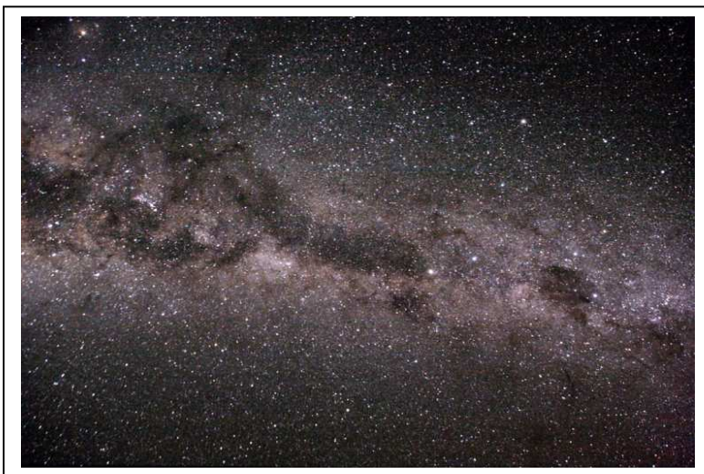
(Left) Milky Way spiral arm: Picture credit - Dieter Willasch
