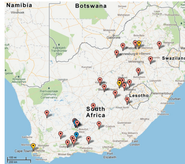
Fig. 6: A map of South Africa marked with the positions of all the testing stations available from the documentation in the SAAO archives. The three yellow pins indicate the existing observatories used for comparison. The blue pins marked the sites that were found to be the best. Source: www.aardvarkmap.net/map/DTSPMO8A where you will be able to browse, zoom and pan into this map.
