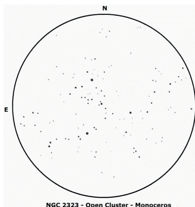
M50; the better known name for NGC 2323 or the Heart Cluster. Photo: D Liebnberg.
