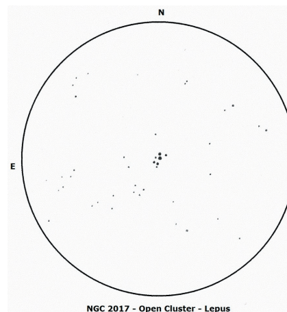
NGC 2017 - Open Cluster - Lepus
