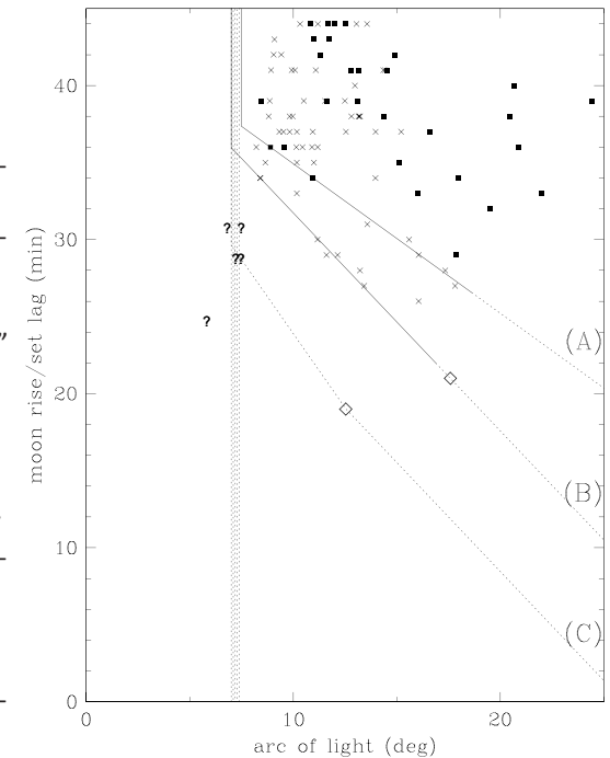
Figure 3. Three criterion lines (A), (B), (C) as described in the text, give interpretation to the crescent visibility implications from combining the moonset lag and the arc of light as indicators.
