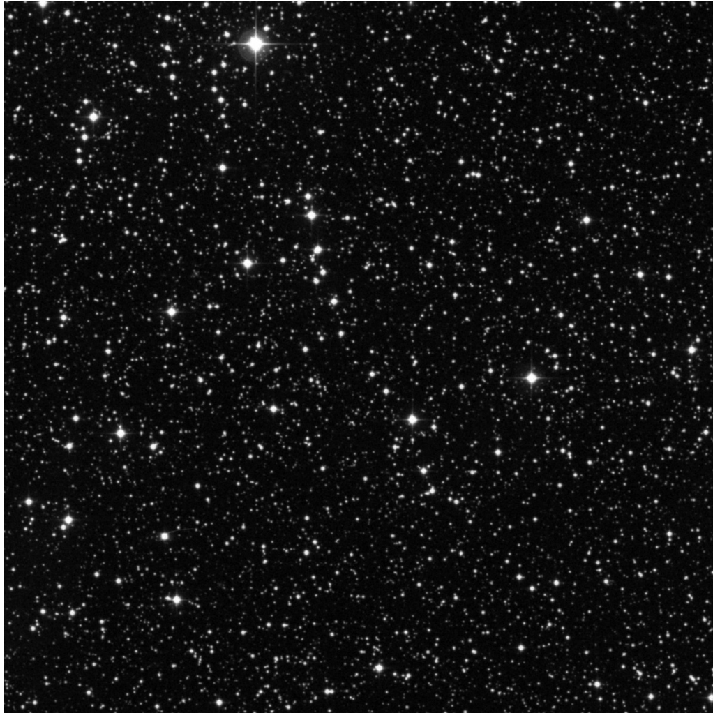
Picture Credit: http://archive.stsci.edu/cgi-bin/dss
