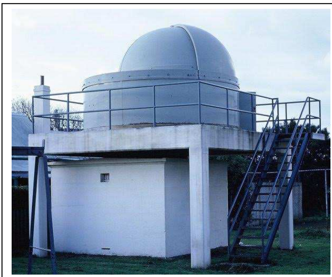
Fig 2. The Cape Kine dome (photo: G. Roberts).
