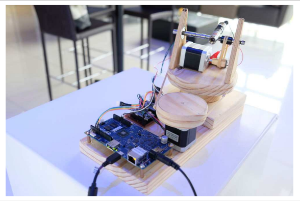
Fig 7. (right) The completed Galileo's Finger
