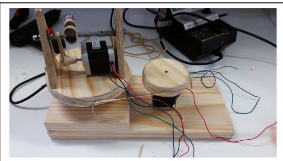
Fig 5. (right) The partly completed Galileo's Finger.
