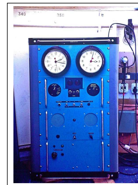
Fig 4. The Cape Kine time unit in 1968 (photo: G Roberts).
