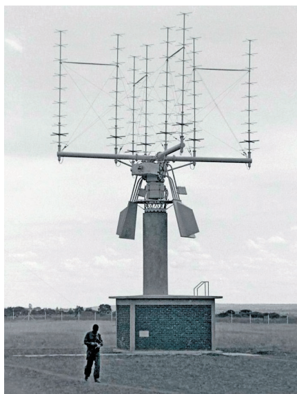
The IRIS antenna – a large array of eight cross-axis yagi antennas used to receive telemetry from satellites operating in the 136-138 Mhz radio band. In addition, commands could be transmitted to the satellite on a frequency close to 148 Mhz. The entire array could be moved in azimuth and altitude to any part of the sky and could follow the satellite as it passed over the station. Picture: Greg Roberts, Easter 1966.
