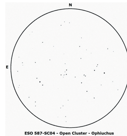
Fig. 2 This cluster displays a close group of five yellowish stars.
