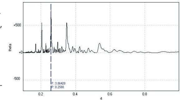
Figure 4: BS Tel V Filter Peranso primary period of P = 0.2588 d
