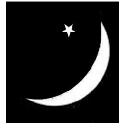
Fig 2. (left) An early image of the "Star and Crescent" that evolved into the modern version.
