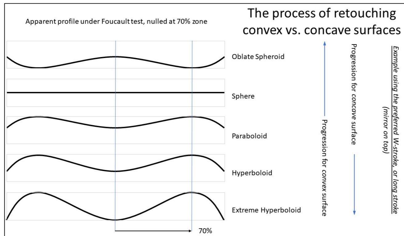
Fig 7. Foucault tests of convex and concave surfaces
