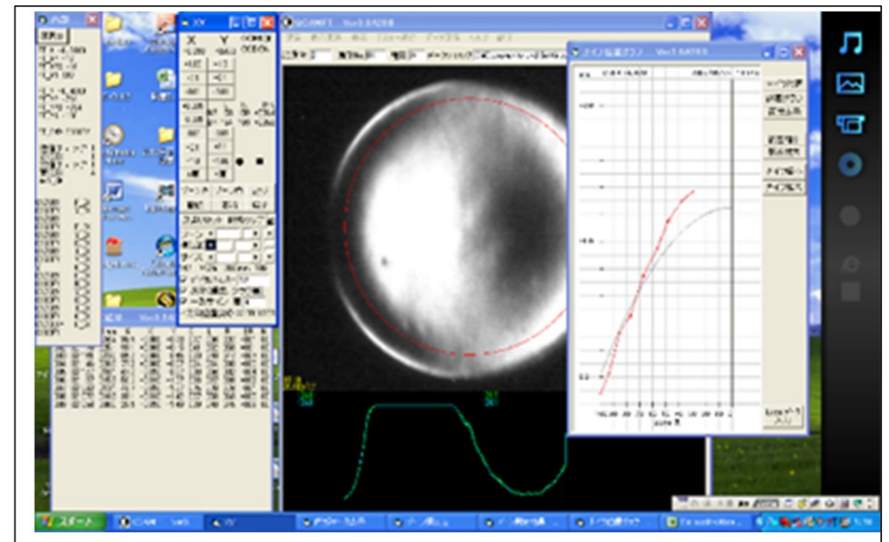
Fig 6. Test measurements and calculations by Auto-Foucault tester. Retouching of Convex surface
