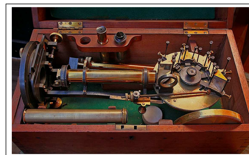
Fig. 3 (below) Five-prism quadruple-pass solar spectrometer from the Thos. Cooke & Sons 1886-1892 design series.
