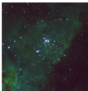
First light image of Trumpler 14, an open cluster and star-forming region near the bright star eta Carina, located about 7050 light years away.
