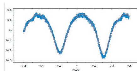
Figure 4: NT Aps V Filter 2008. Fitted the phase binned.
