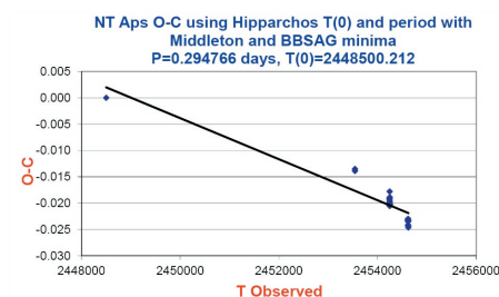
Figure 2: O-C Diagram using Hipparcos T_0 and period including BBSAG and Middleton minima.
