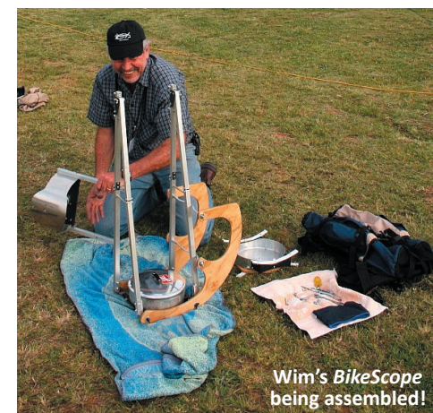
Wim Filmalter's 8-inch BikeScope, which fits into his backpack packed.
