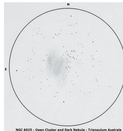
NGC 6025 - Open Cluster and Dark Nebula - Triangulum Australe
