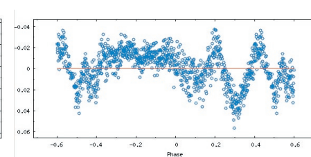
Figure 5: NT Aps residuals of the synthetic light curve (red) on PHOEBE model.
