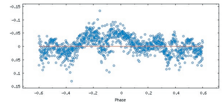
Figure 5: UV Grus residuals of the synthetic light PHOEBE model.
